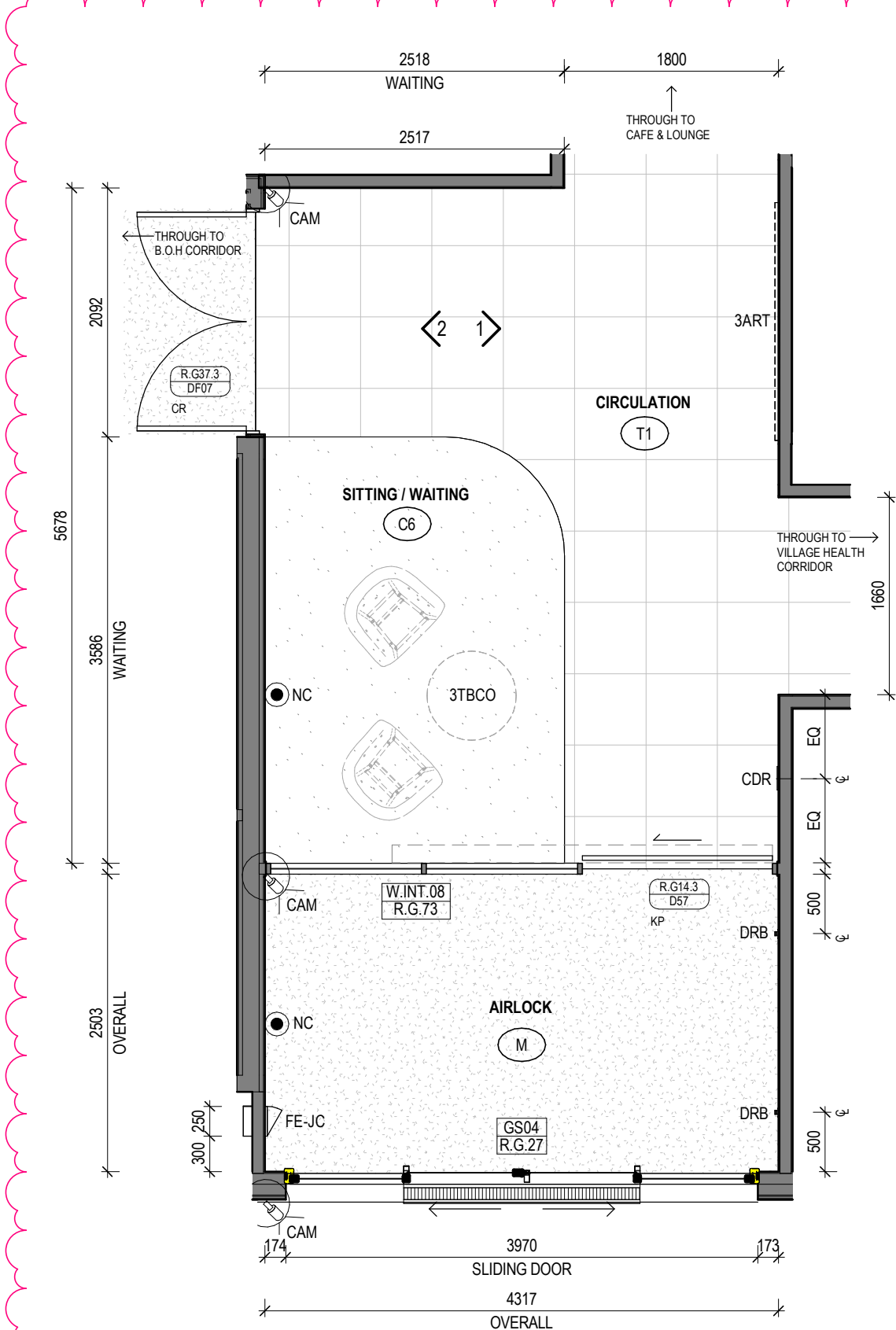
5 VILLAGE HEALTH & WELLNESS - AIRLOCK & WAITING Scale 1: 50
