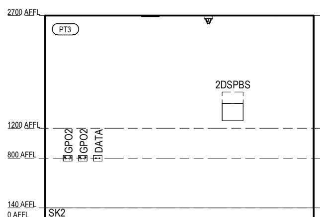
VILLAGE HEALTH & WELLNESS - CONSULT 2 ELEVATION 1 Scale 1: 50
