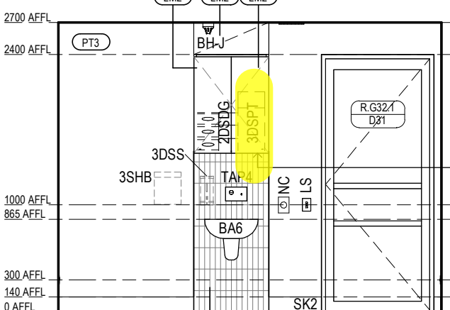
VILLAGE HEALTH & WELLNESS - CONSULT 2 ELEVATION 3 Scale 1: 50
