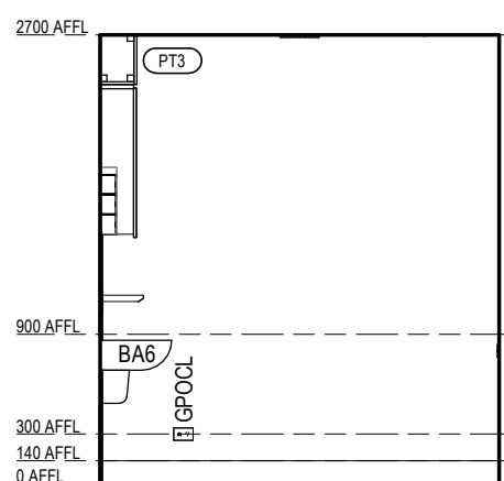
VILLAGE HEALTH & WELLNESS - CONSULT 2 ELEVATION 4 Scale 1: 50
