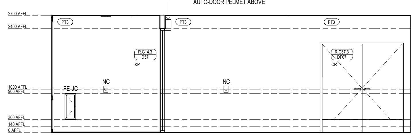
VILLAGE HEALTH & WELLNESS - AIRLOCK & WAITING ELEVATION 2 Scale 1: 50
