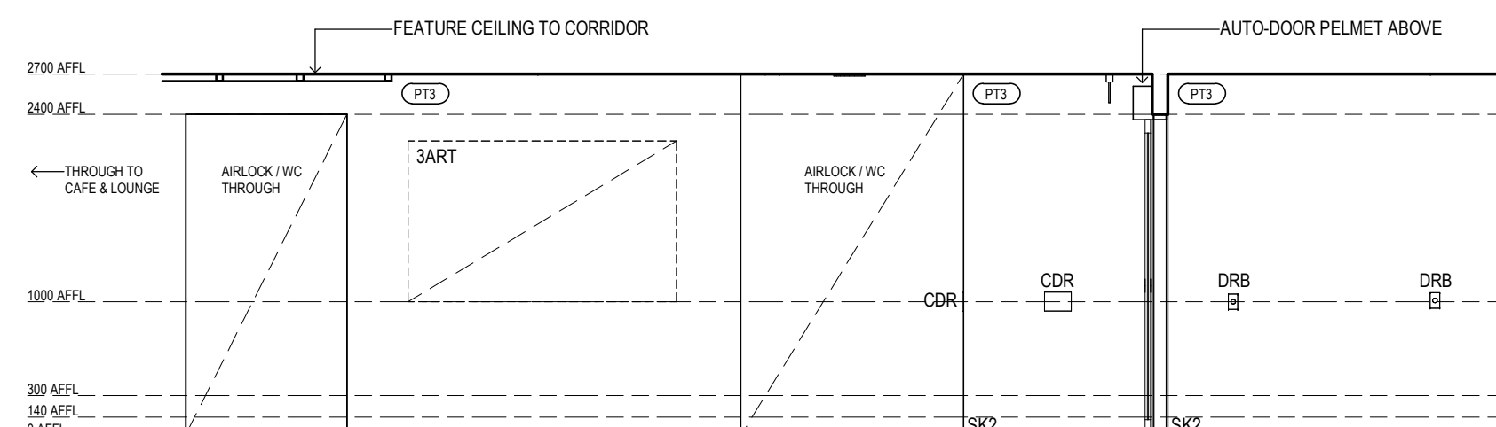
VILLAGE HEALTH & WELLNESS - AIRLOCK & CIRCULATION ELEVATION 1 Scale 1: 50
