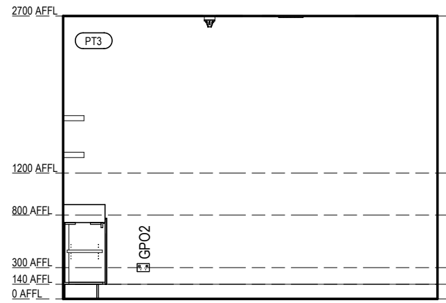
VILLAGE HEALTH & WELLNESS - CONSULT 1 ELEVATION 1 Scale 1: 50
