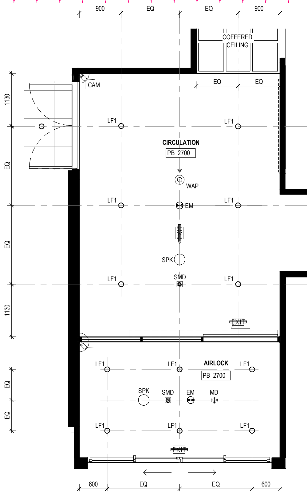
6 RCP - VILLAGE HEALTH & WELLNESS - AIRLOCK & WAITING Scale 1: 50
