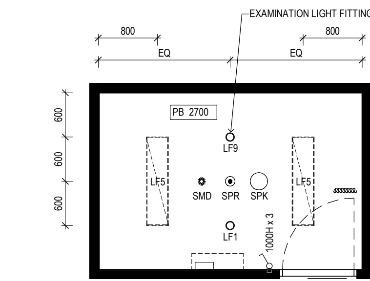
2 RCP - VILLAGE HEALTH & WELLNESS - CONSULT 1 Scale 1: 50
