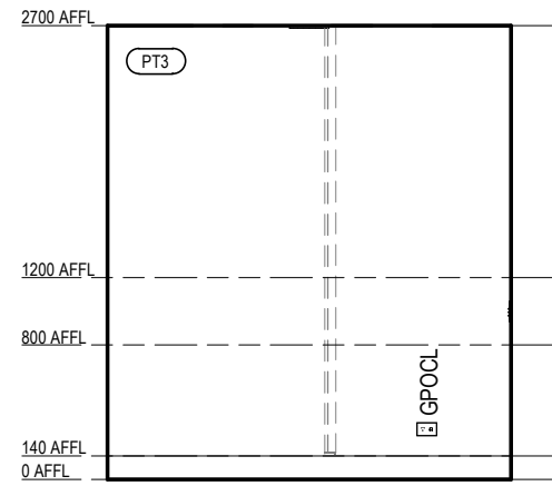
VILLAGE HEALTH & WELLNESS - CONSULT 1 ELEVATION 2 Scale 1: 50
