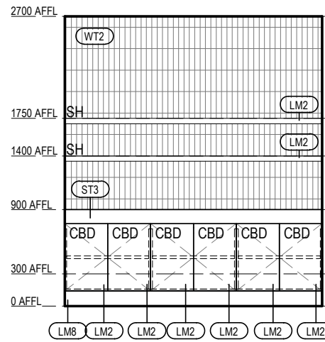
VILLAGE HEALTH & WELLNESS - CONSULT 1 ELEVATION 4 Scale 1: 50
