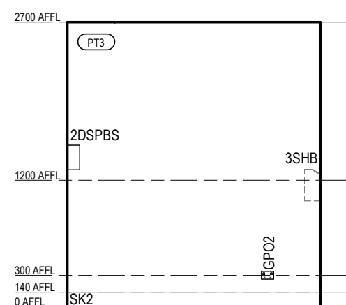
VILLAGE HEALTH & WELLNESS - CONSULT 2 ELEVATION 2 Scale 1: 50
